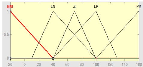
Fig. 4: Membership functions for input variable E(k)
