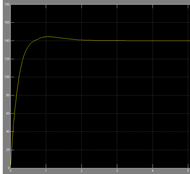
Fig. 10: Speed Vs time response of controlled DC motor
