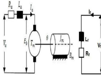
Fig 1: DC motor
