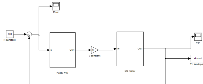
Fig. 9: Simulink Model Implemented
